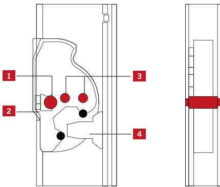
Disengaged lock
